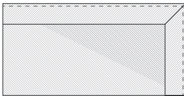
SECTION CR: TOP VIEW 80w x 40d x 23.5h Leather: 140 sq ft Fabric: 11 yards
